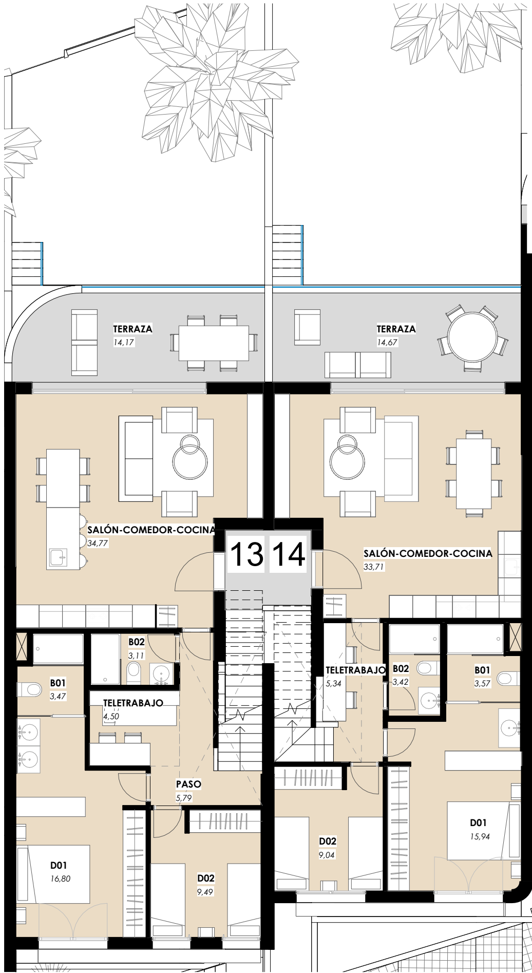
VIVIENDA 13-14_PLANTA PRIMERA/ APARTMENT 13-14_TOP FLOOR
