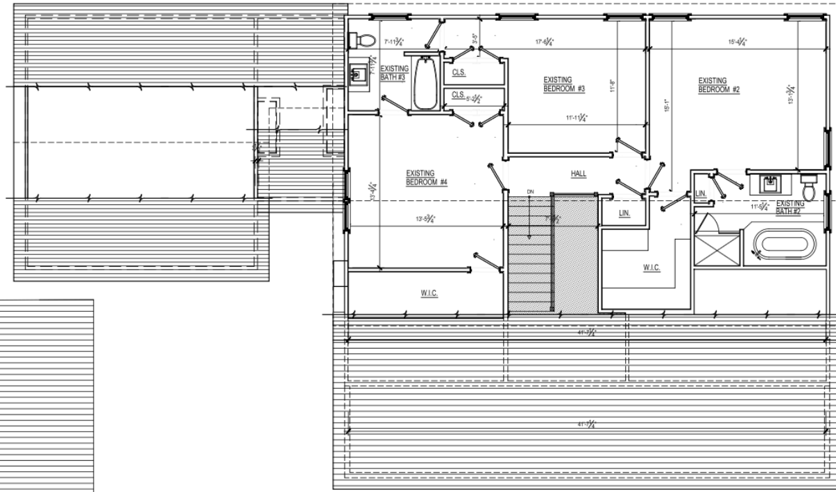
EXISTING SECOND FLOOR PLAN SCALE: 1/4" = 1'-0"
